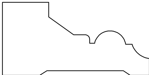
CA-208 1 1/4" X 2 1/2"
