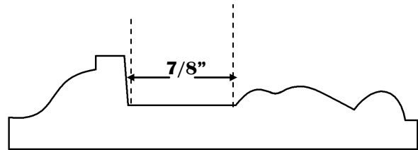
CHR-301 11/16" X 3"
