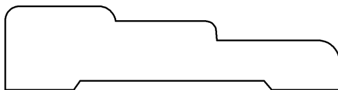
CA-210 5/8" X 2 1/2"
