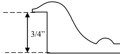
BC-002 7/8" X 1 1/2"
