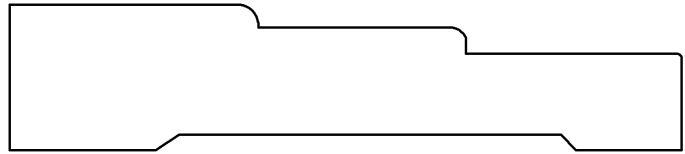
CA-312 3/4" X 3 1/2"
