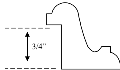
BC-102 1 1/8" X 1 1/4"
